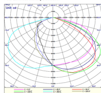
Polar Luminous Intensity Distribution
