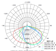
INTENSITY DISTRIBUTION DIAGRAM IN C-PLANE
