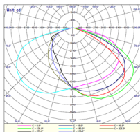
Polar Luminous Intensity Distribution
