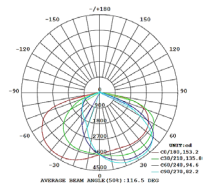
INTENSITY DISTRIBUTION DIAGRAM IN C-PLANE
