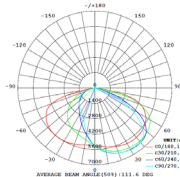
INTENSITY DISTRIBUTION DIAGRAM IN C PLANE
